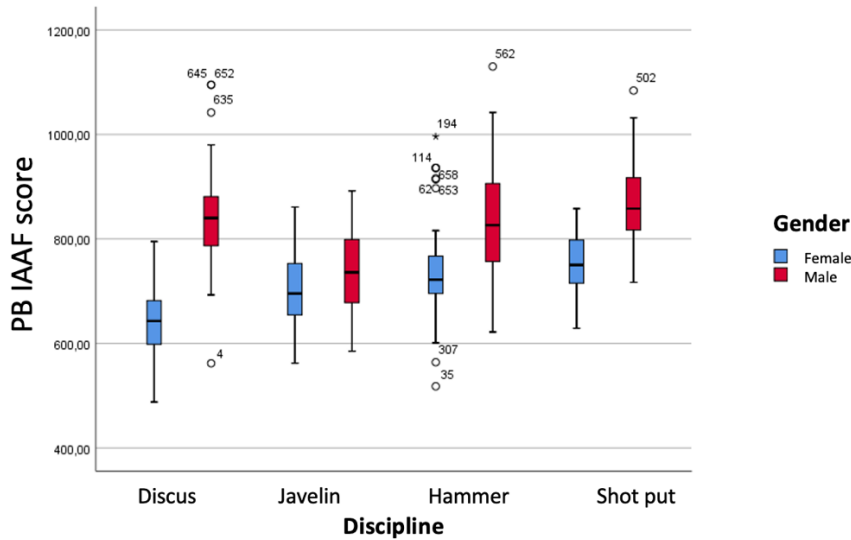
Figure 1. Distribution of athletes according to gender, category and performance.
